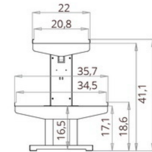
SUPER STRUCTURE with LED LIGHT P : 2100 MM P : 2500 MM
